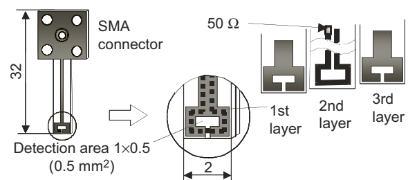
Fig. 3 Near magnetic probe
