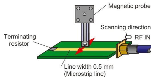
Fig. 6 Method of measuring frequency characteristic and resolution
