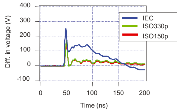
(a) Difference in voltage across the terminating resistor w/o capacitor
